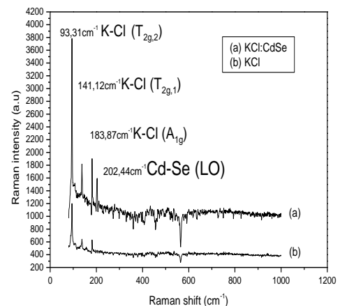
Fig 4: \mu -Raman spectra: (a) pure KCl (b) KCl:CdSe.
